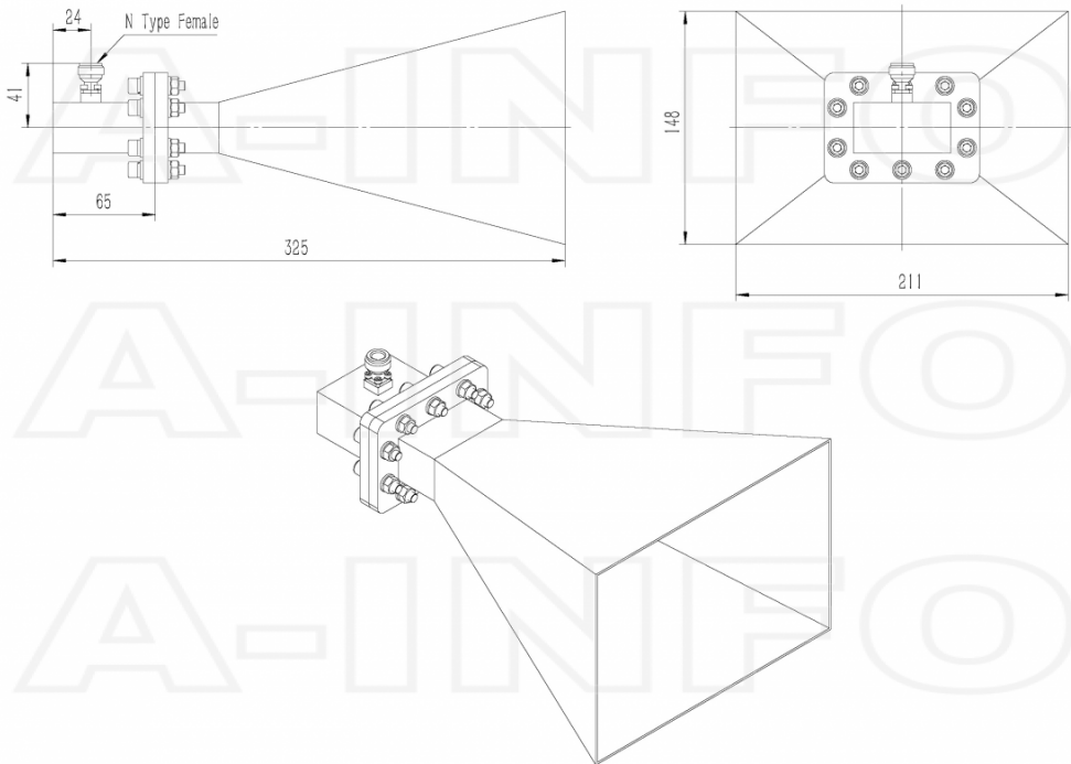
N-Female Output (P/N: LB-229-15-C-NF)
